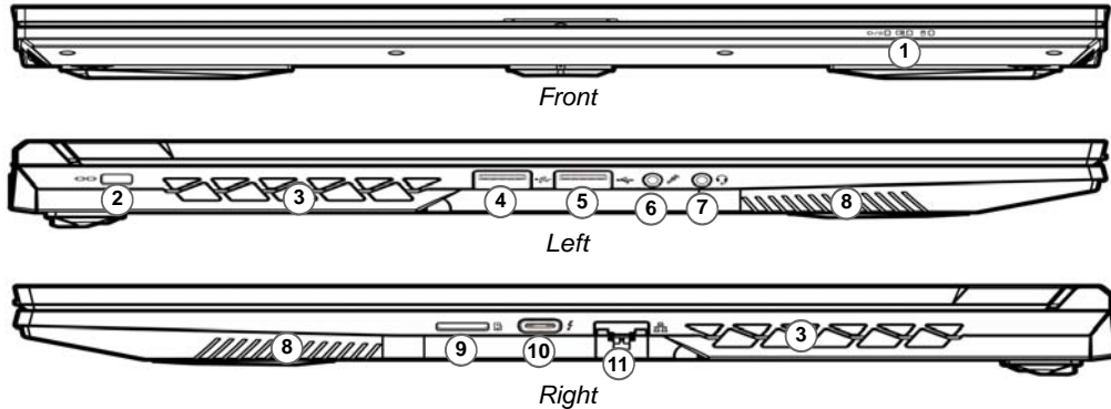
Figure 5 Front, Left & Right Views (Model C)
