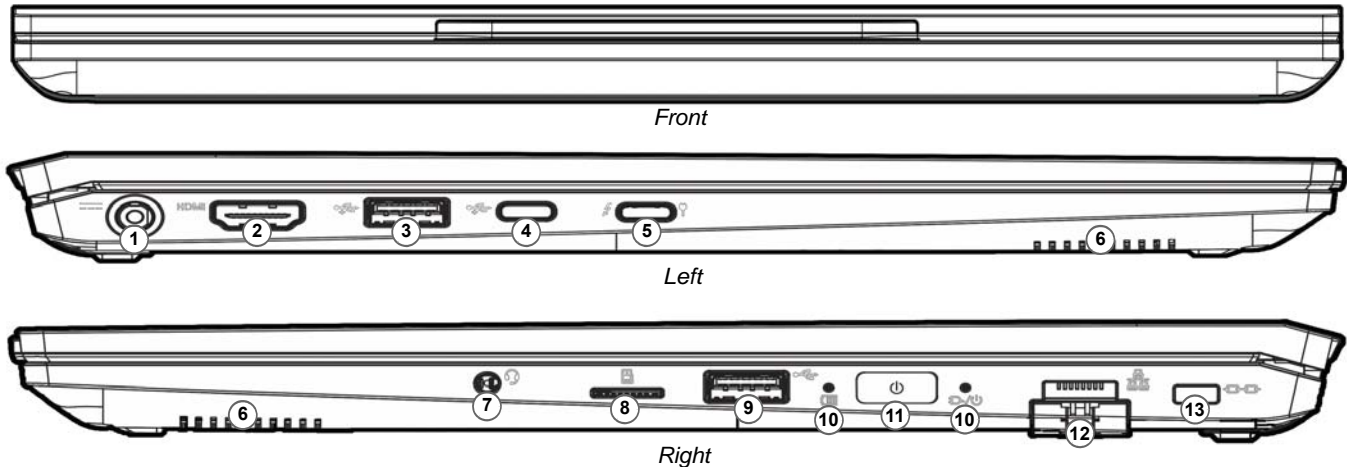
Figure 4 - Front, Left & Right Views (Model A)
