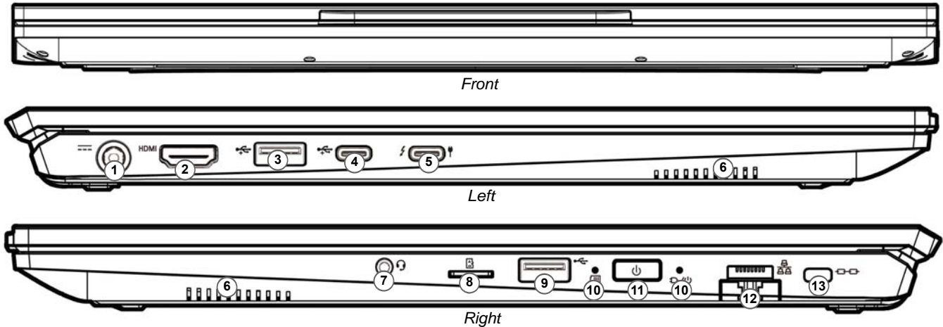
Figure 5 - Front, Left & Right Views (Model B)
