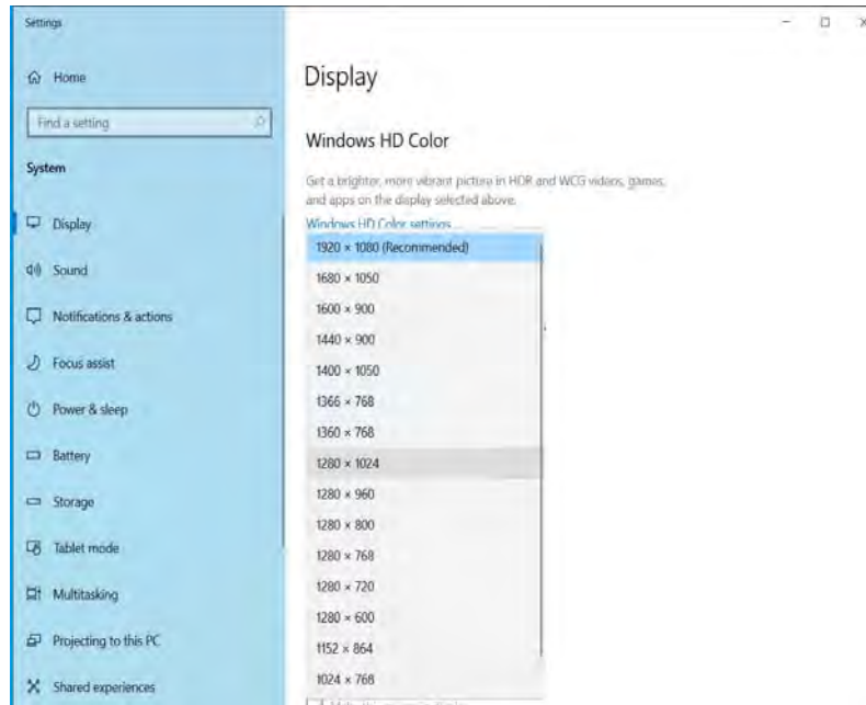
Figure 1 - 24 - Display (Resolution)
