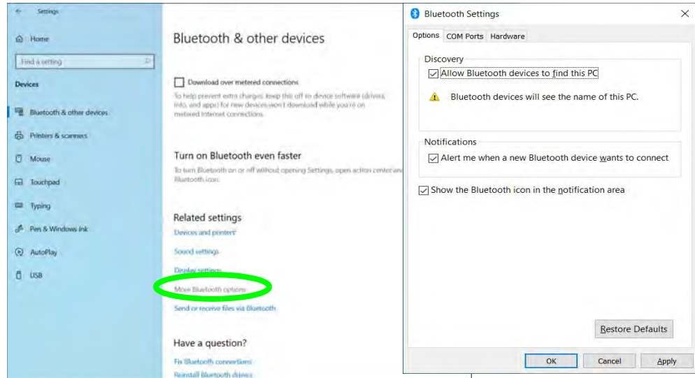
Figure 6 - 8 Bluetooth Settings
