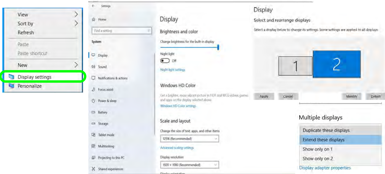
Figure 1 - 22 - Display Settings
