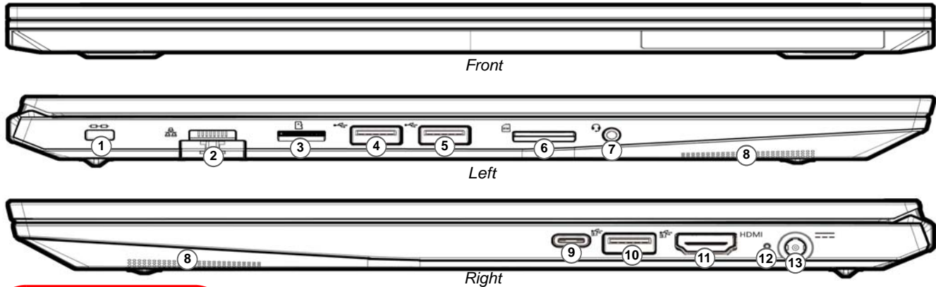
Figure 12 - Front, Left & Right Views (Model B)
