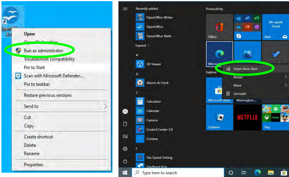
Figure 1 - 11 - Pin to Start/Unpin from Start
