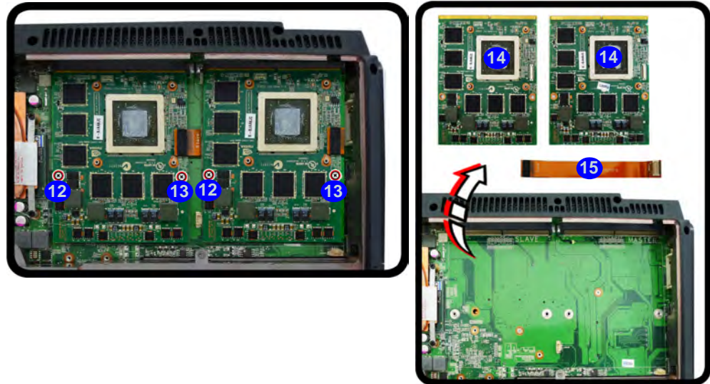
Figure 6 - 24 Video Card Removal
