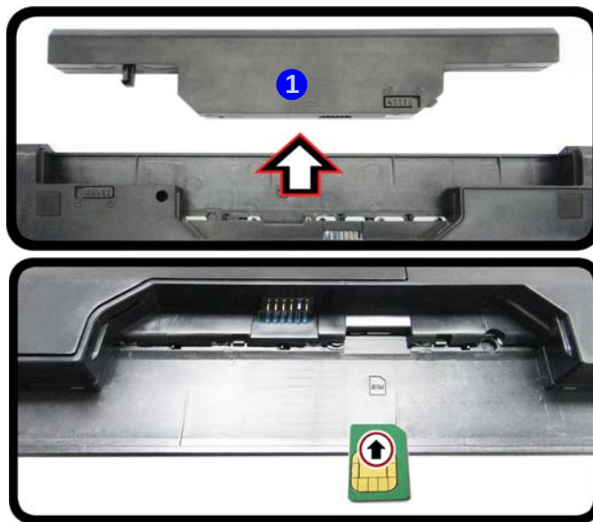
Figure 15 - Remove the battery and Insert the USIM Card
