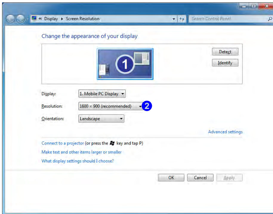
Figure 1 - 9 - Screen Resolution
