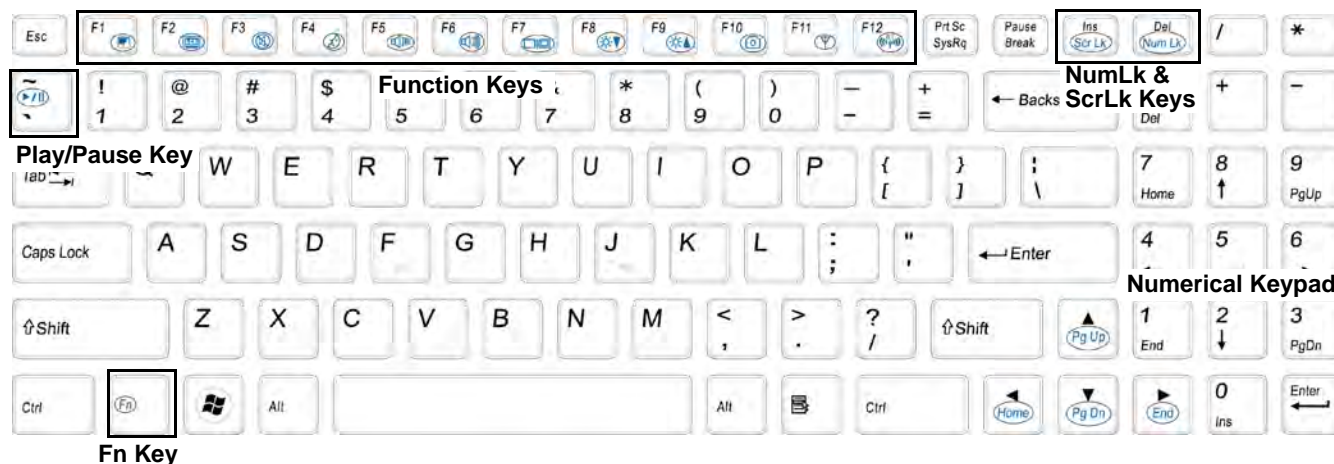
Figure 1 - 4 - Keyboard
