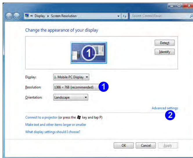
Figure 1 - 11 - Screen Resolution
