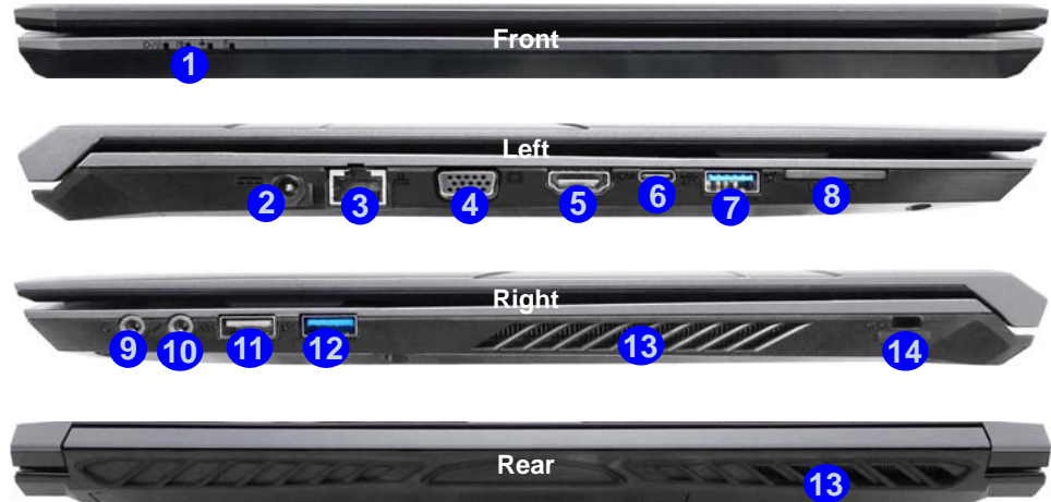
Figure 15 - Front, Left, Right & Rear Views (Model B)
