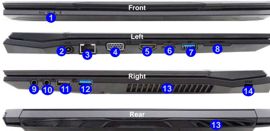
Figure 14 - Front, Left, Right & Rear Views (Model A)
