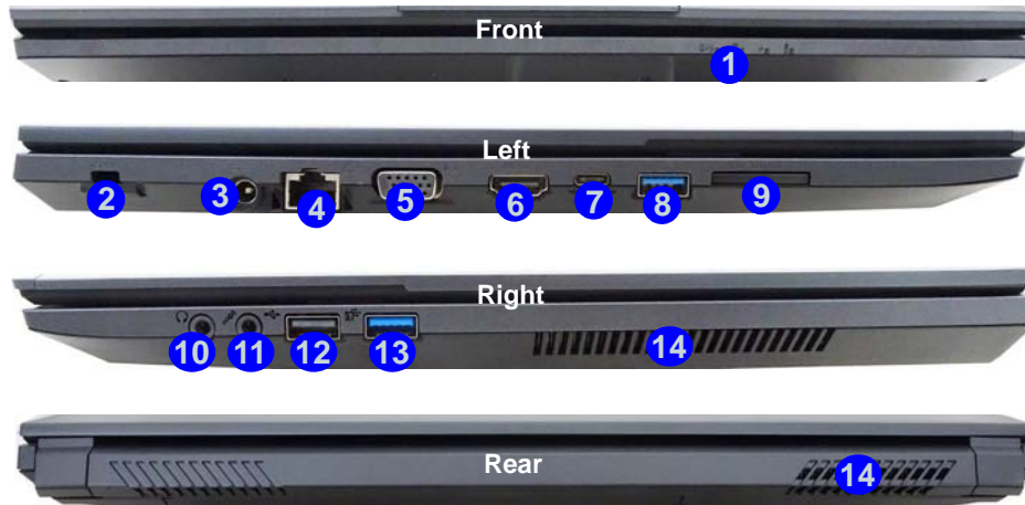
Figure 16 - Front, Left, Right & Rear Views (Model C)
