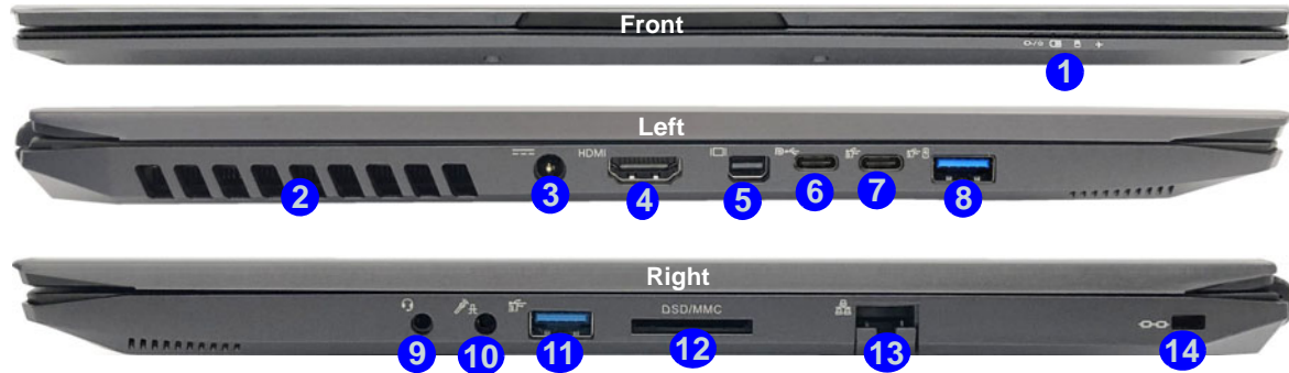
Figure 5 - Front, Left & Right Views (Model C)
