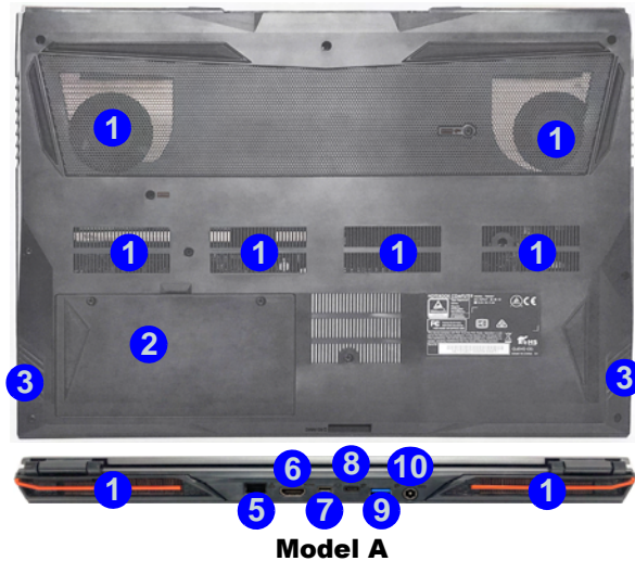
Figure 5 - Bottom & Rear Views
