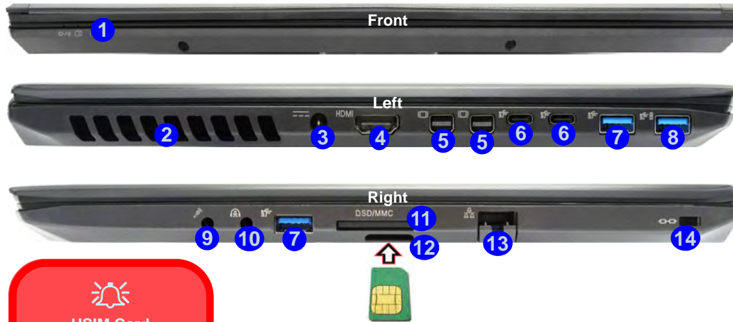
Figure 5 - Front, Left & Right Views (Model A)
