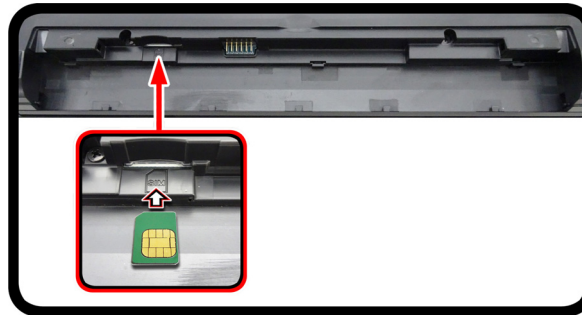
Figure 17 - Remove the battery and Insert the USIM Card
