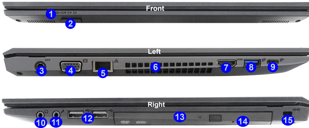
Figure 7 - Front, Left & Right Views (Model A)
