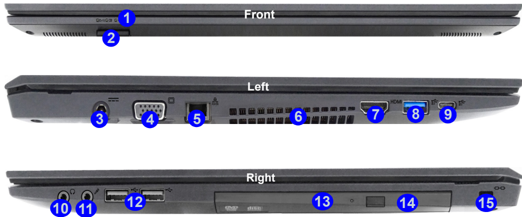
Figure 8 - Front, Left & Right Views (Model B)
