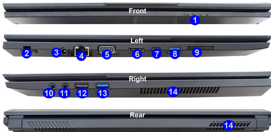
Figure 9 - Front, Left, Right & Rear Views (Model C)
