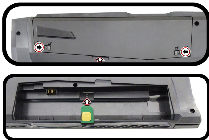
Figure 27 - Remove the battery and Insert the USIM Card
