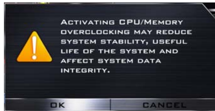
Figure 12 - CPU Overclocking
