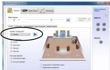
Figure 31 Speaker Configuration
