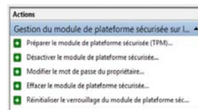
Figure 37 Menu Actions
