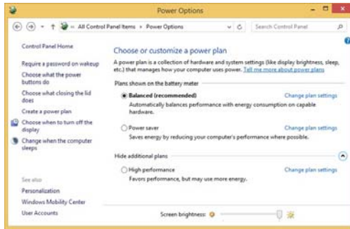
Figure 30 - Power Options
