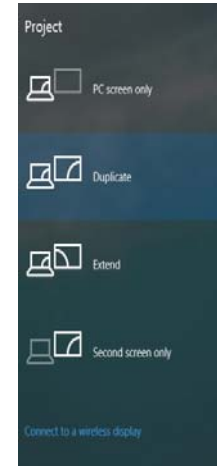
Figure 28 Project
