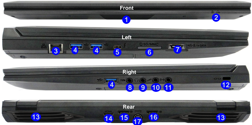
Figure 18 Front, Left, Right & Rear Views (Model A)
