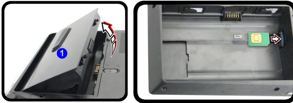
Figure 33 - Remove the battery and Insert the USIM Card
