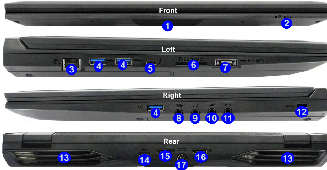
Figure 19 Front, Left, Right & Rear Views (Model B)
