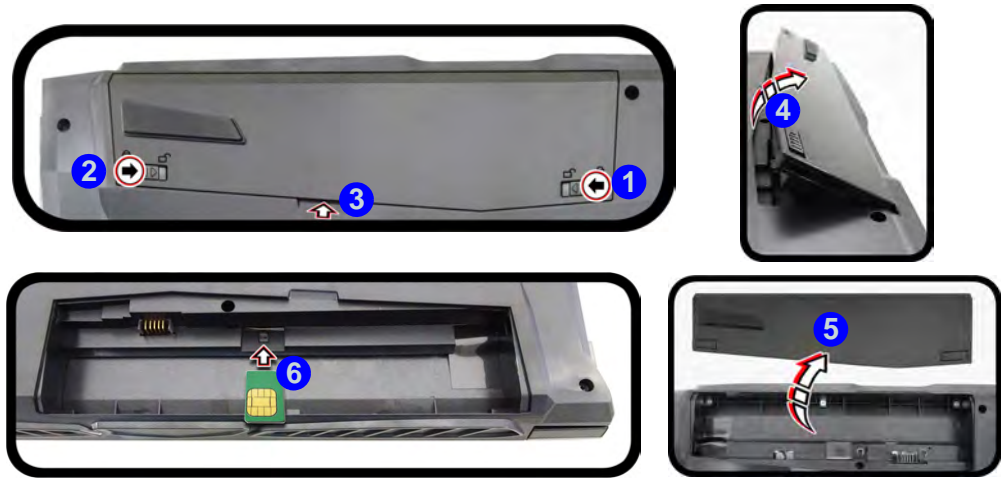
Figure 6 - 50 Battery Removal & USIM Card Insertion
