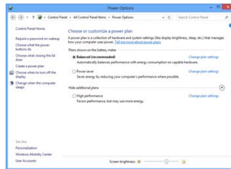
Figure 18 - Power Options
