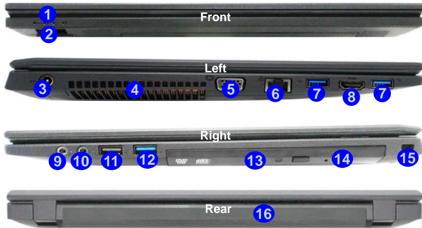
Figure 13 - Front, Left, Right & Rear Views (Model A)
