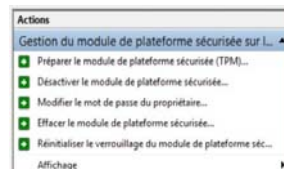
Figure 23 Menu Actions
