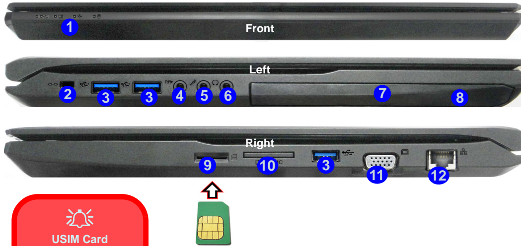
Figure 13 - Front, Left & Right Views (Model B)
