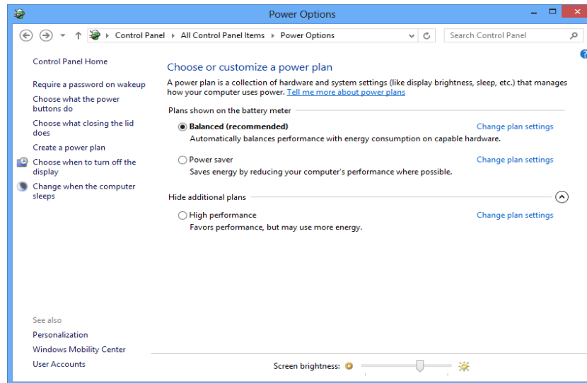
Figure 22 - Power Options
