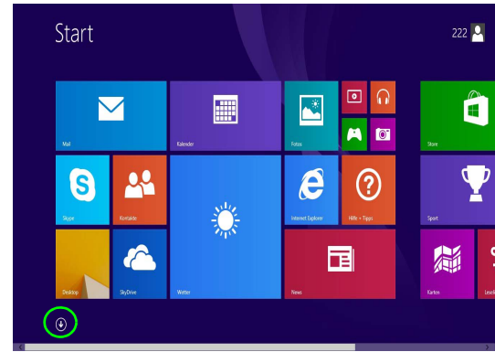
Abb. 17 - Start-Bildschirm (Windows 8.1)
