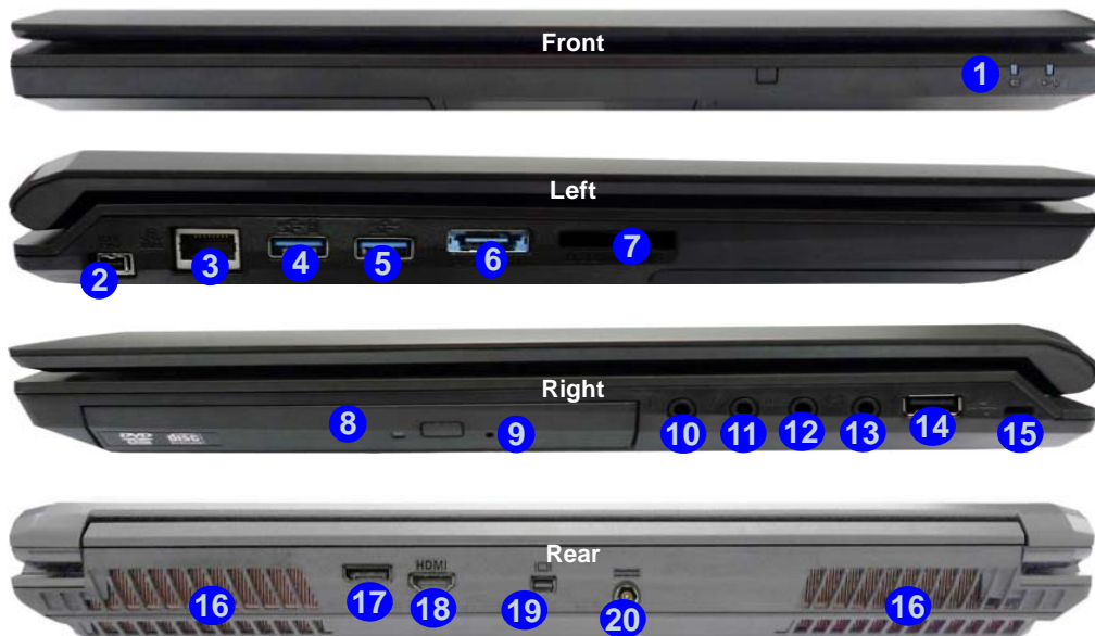
Figure 12 Front, Left, Right & Rear Views (Models A, C & D)
