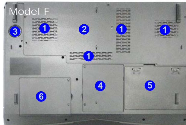
Figure 16 Bottom Views (Models E & F)
