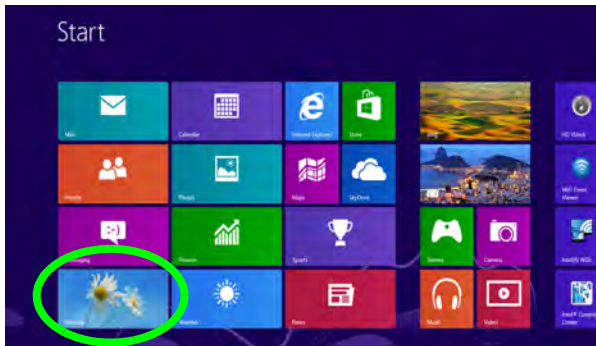
Figure 7 Start Screen
