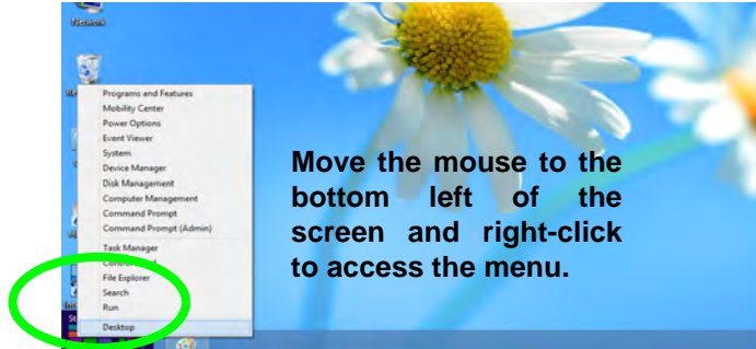
Figure 6 Context Menu
