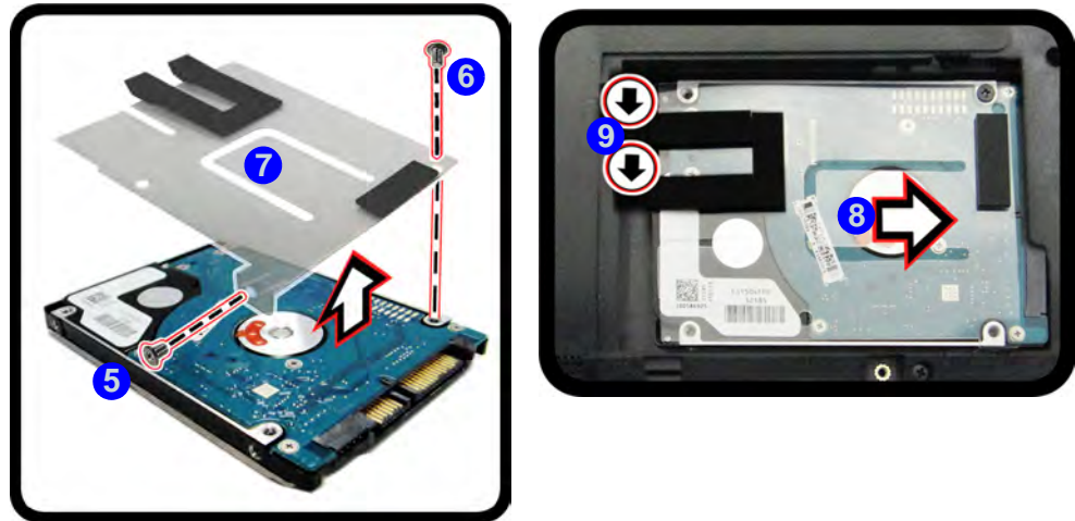
Figure 6 - 5 Hard Disk Assembly Cover and Screws Removal / Hard Disk Assembly Insertion
