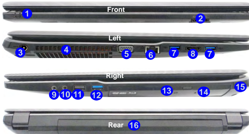
Figure 15 - Front, Left, Right & Rear Views (Model B)
