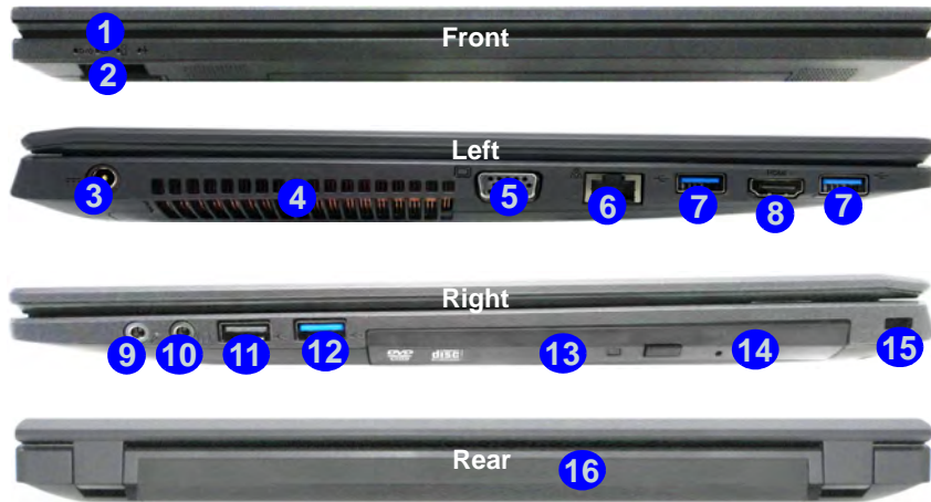
Figure 14 - Front, Left, Right & Rear Views (Model A)
