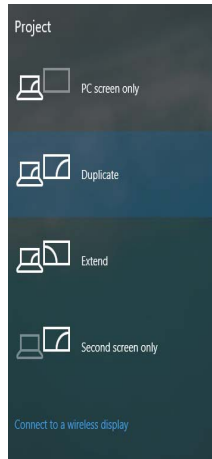
Figure 17 Project
