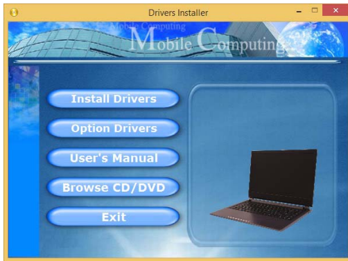
Figure 20 - Install Drivers
