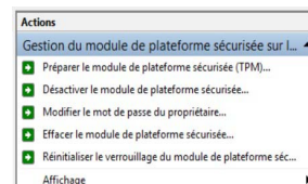
Figure 23 Menu Actions
