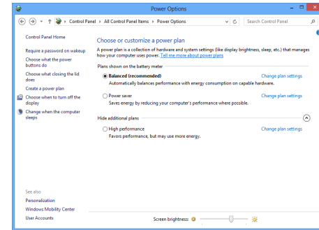
Figure 18 - Power Options
