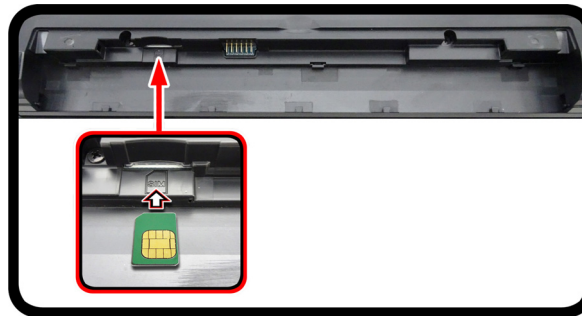
Figure 15 - Remove the battery and Insert the USIM Card
