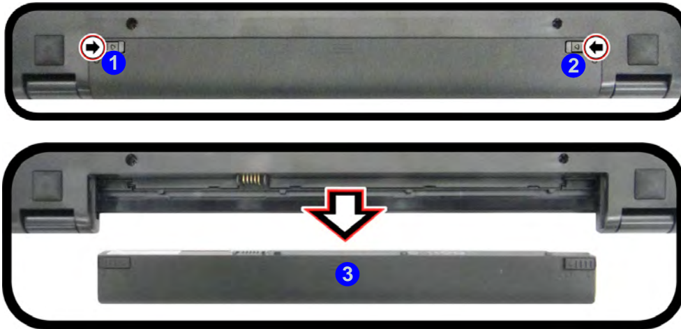
Figure 1 - 18 Battery Removal Model C Computers
