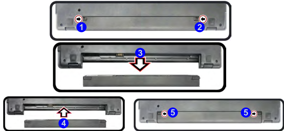
Figure 3 - 16 Battery Removal for Model B Computers
