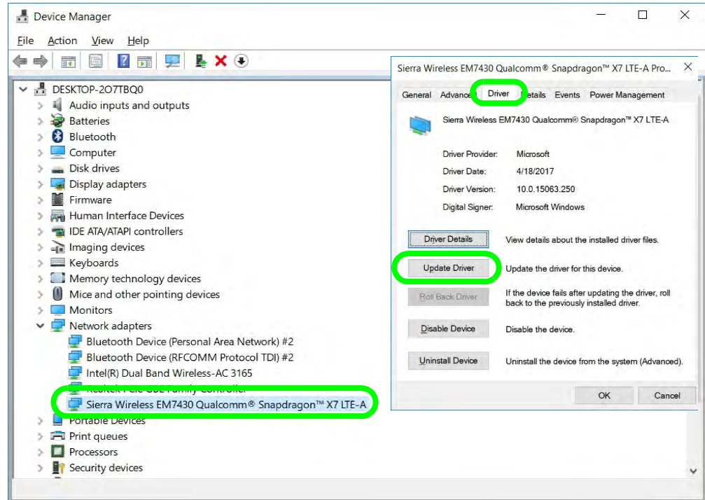
Figure 6 - 37 Device Manager Network Adapters
